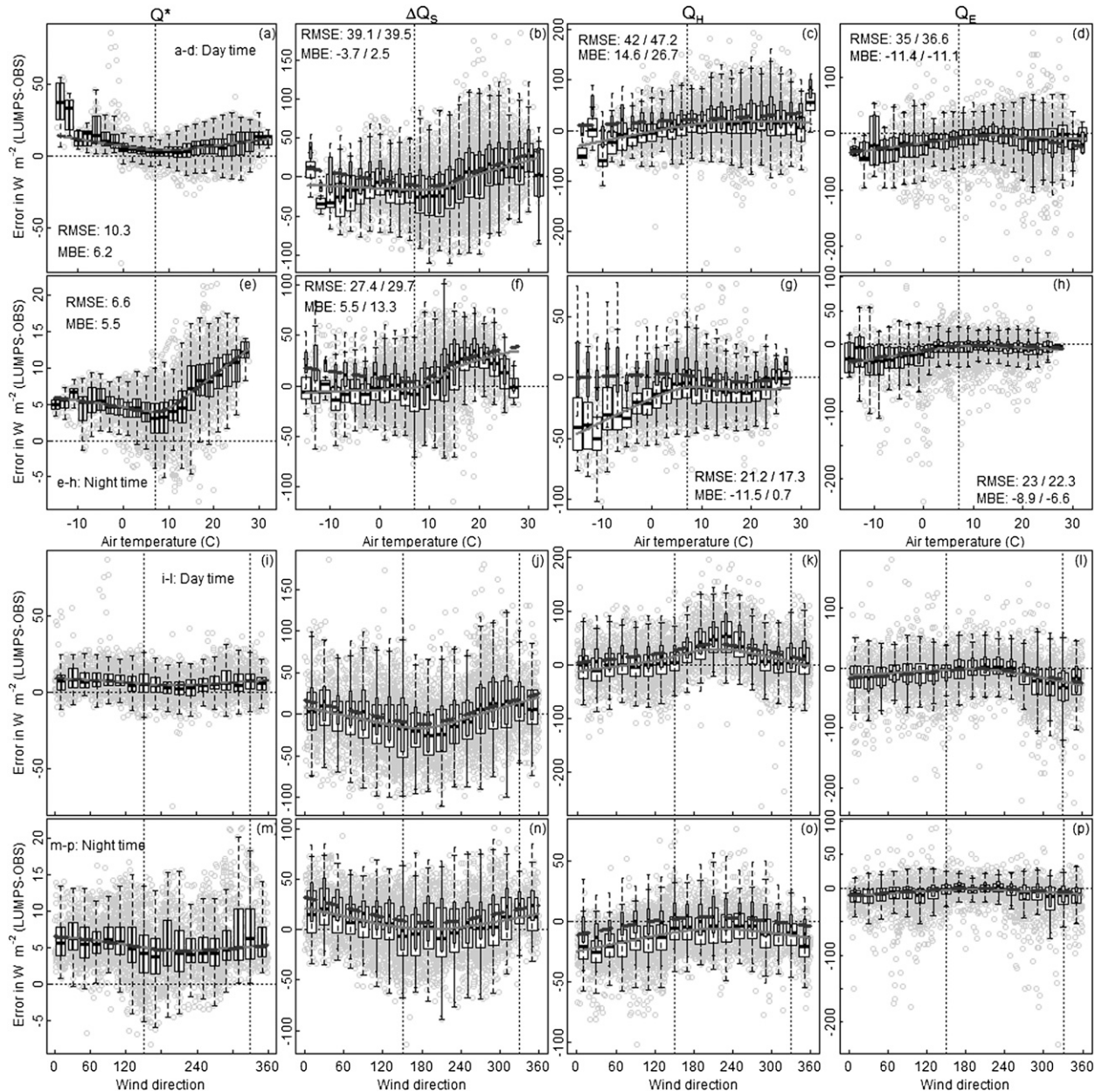
FIG. 9. Error [(a)–(d),(i)–(l) daytime and (e)–(h),(m)–(p) nighttime] between modeled (using L \downarrow option 1) and observed values of Q^* , \Delta Q_S , Q_H , and Q_E for the 2-yr period as a function of (top and top middle) air temperature and (bottom and bottom middle) wind direction. Lower lines for base run (solid) and run 2 ( Q_F , changing surface characteristics) (dashed). Box plots (white—wider for the base run; gray—narrower run 2) are for bins of 2^\circ\text{C} temperature for (a)–(h) and 20^\circ wind direction for (i)–(p). RMSE and MBE statistics are indicated in (a)–(h) for base run (left) and run 2 (right). For Q^* , both runs are the same. See text for definition of the vertical threshold (dashed) lines.
